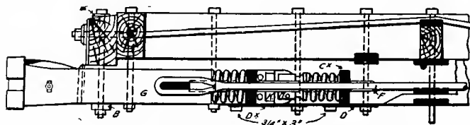
Fig. 1941. Sectional Side Elevation. THE IMPROVED AMERICAN DRAFT AND BUFFING APPARATUS. Letters refer to details below.
